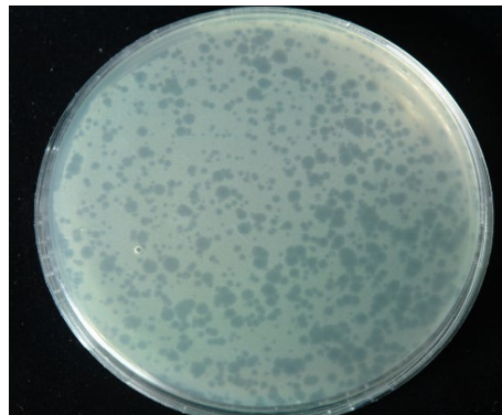
Fig 3: Plaques observed after infecting E. coli with lambda phage
